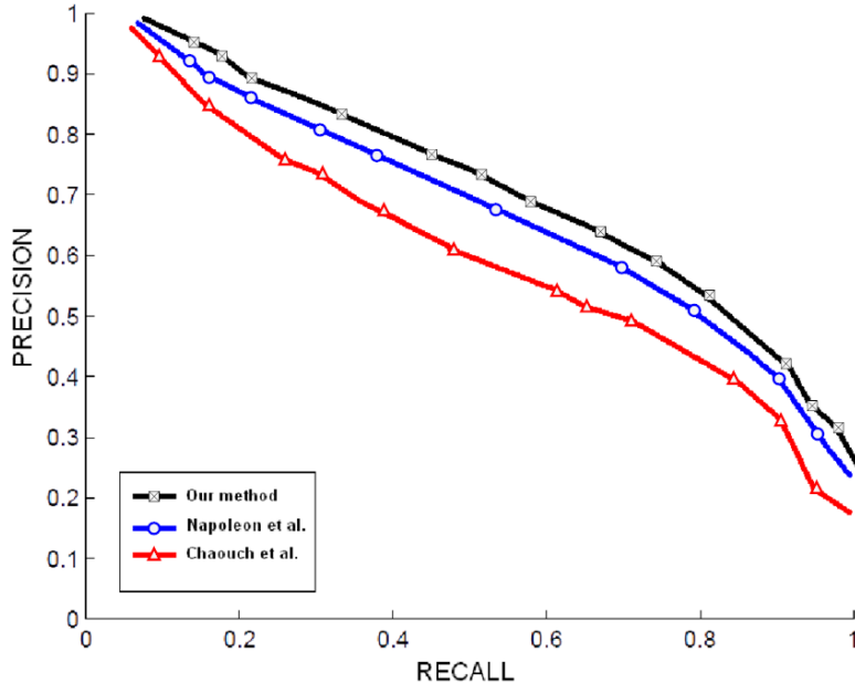
Figure 3. Precision vs Recall plots for our method and some stat of art methods On the Shrec07 dataset.
